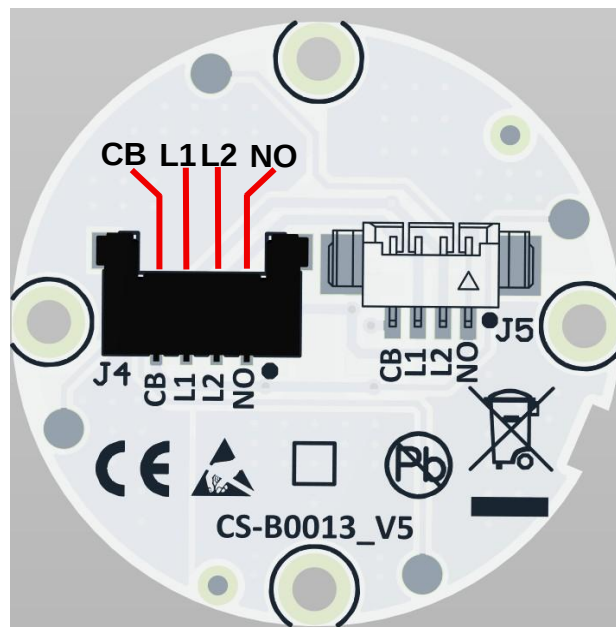
Pico-Lock connector/ Connettore Pico-Lock
