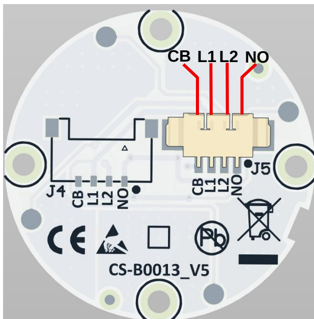
PicoBlade connector/ Connettore PicoBlade
