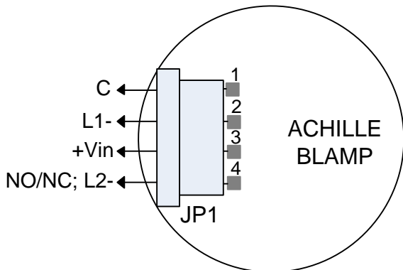
AMP connector/ Connettore AMP
